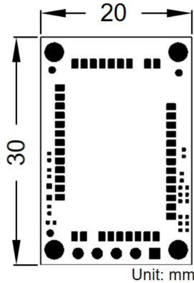
Figure 5: Mechanical Dimensions
