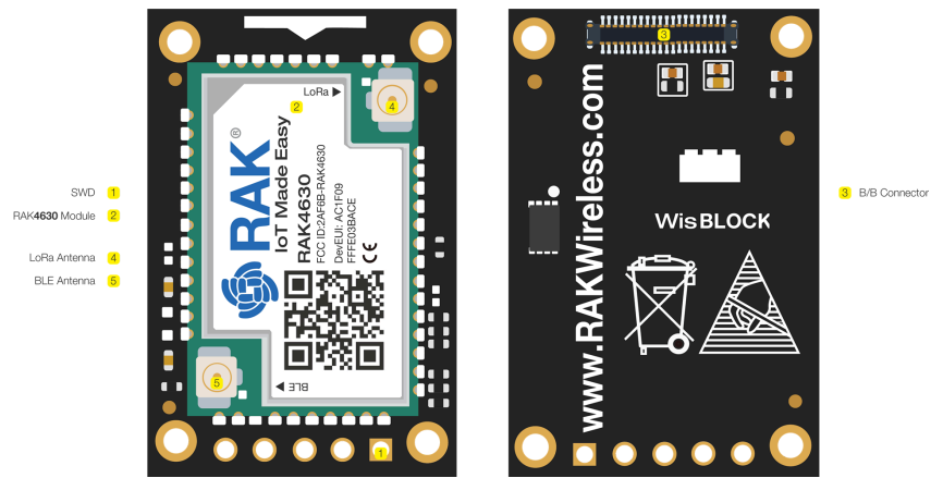
Figure 1: RAK4631 Overview
