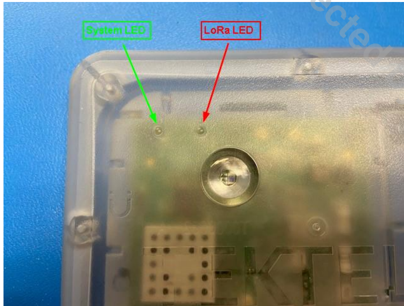
Figure 8 LED Location
