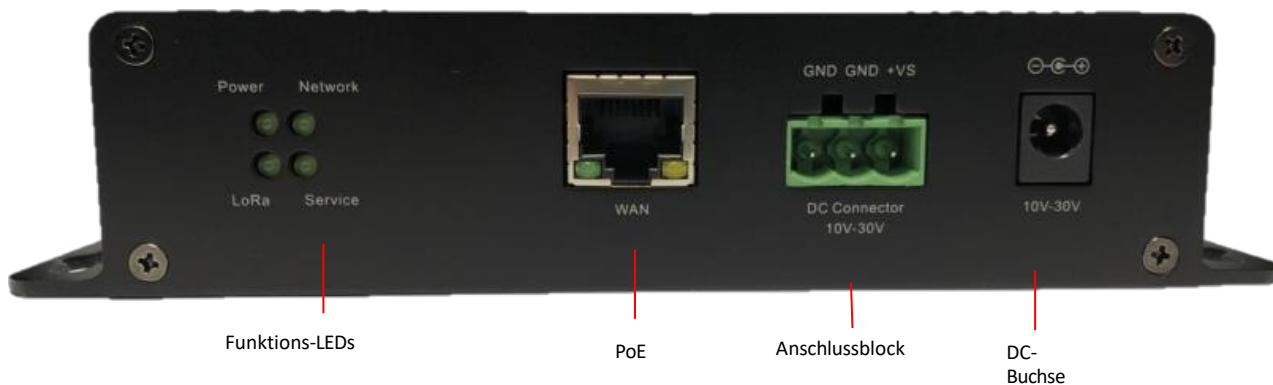
Frontplatte
