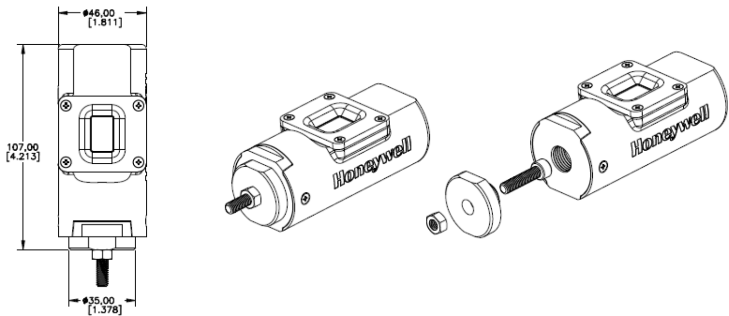
Figure 7– Screw mount
