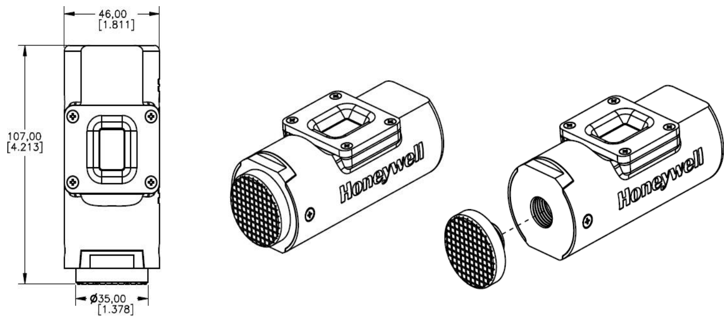
Figure 8– Epoxy Mount
