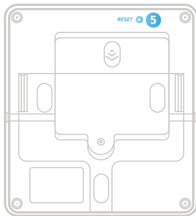
Assembled MClimate Wireless Thermostat LoRaWAN®, bottom view
