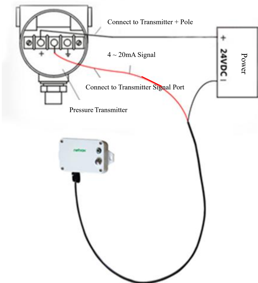
Figure1 2-wire System Example Diagram (for wiring reference)
