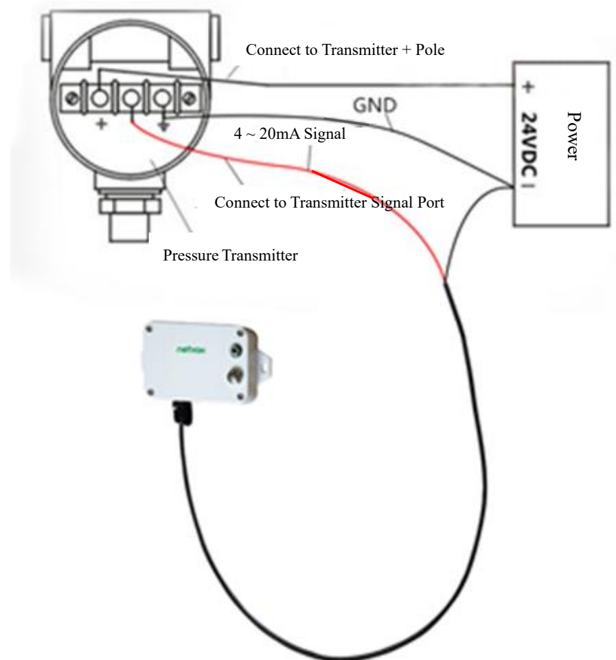
Figure2 3-wire System Example Diagram (for wiring reference)
