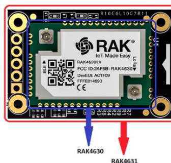
Figure 1: RAK4631 Overview
