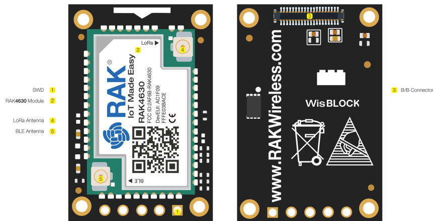
Figure 1: RAK4631 Overview
