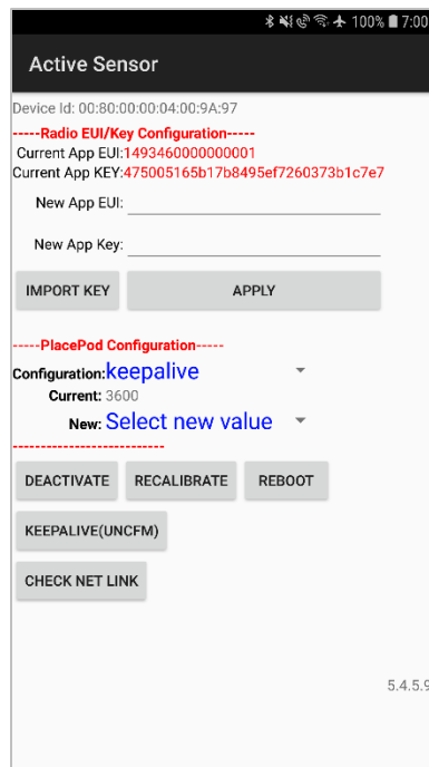
Figure 10: Set Network Keys
